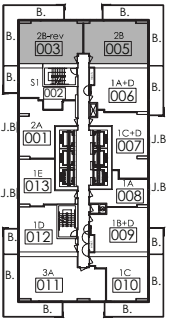
KEYPLAN 20-22ND, 27TH, 29TH, 34-35TH
