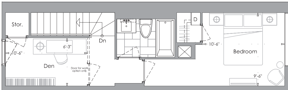
Upper Floor-Live 390 sq. ft.
