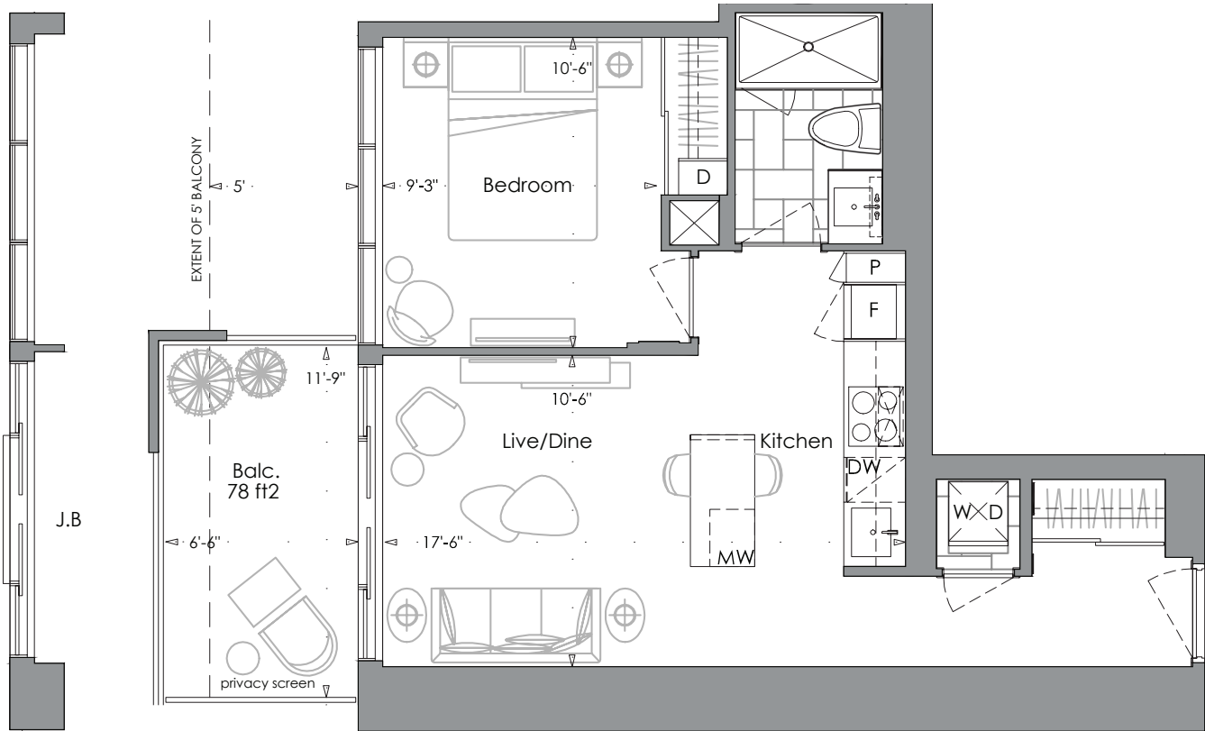
Juliet Balcony Layout
