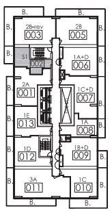
KEYPLAN 38-40TH
